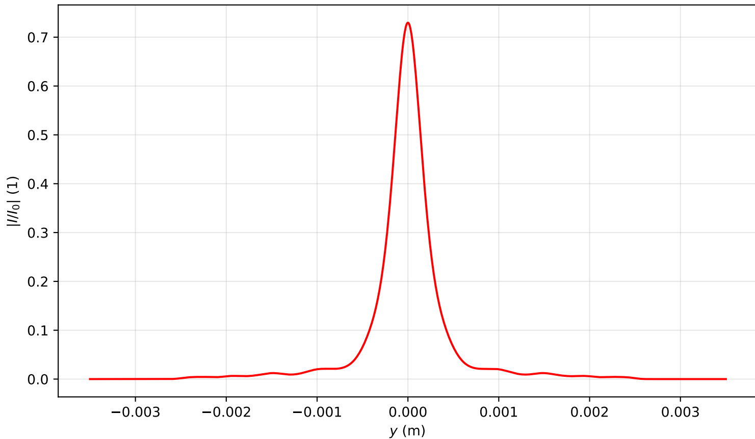
Intensity profile I(x=0, y, z=3.344)/I_0 , P_{in}=3.0P_{cr} , artificial time
